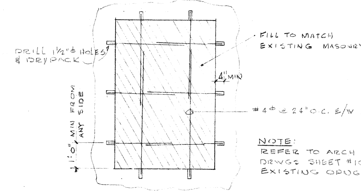
CLOSE EXISTING MASONRY OPNGS. NO SCALE
