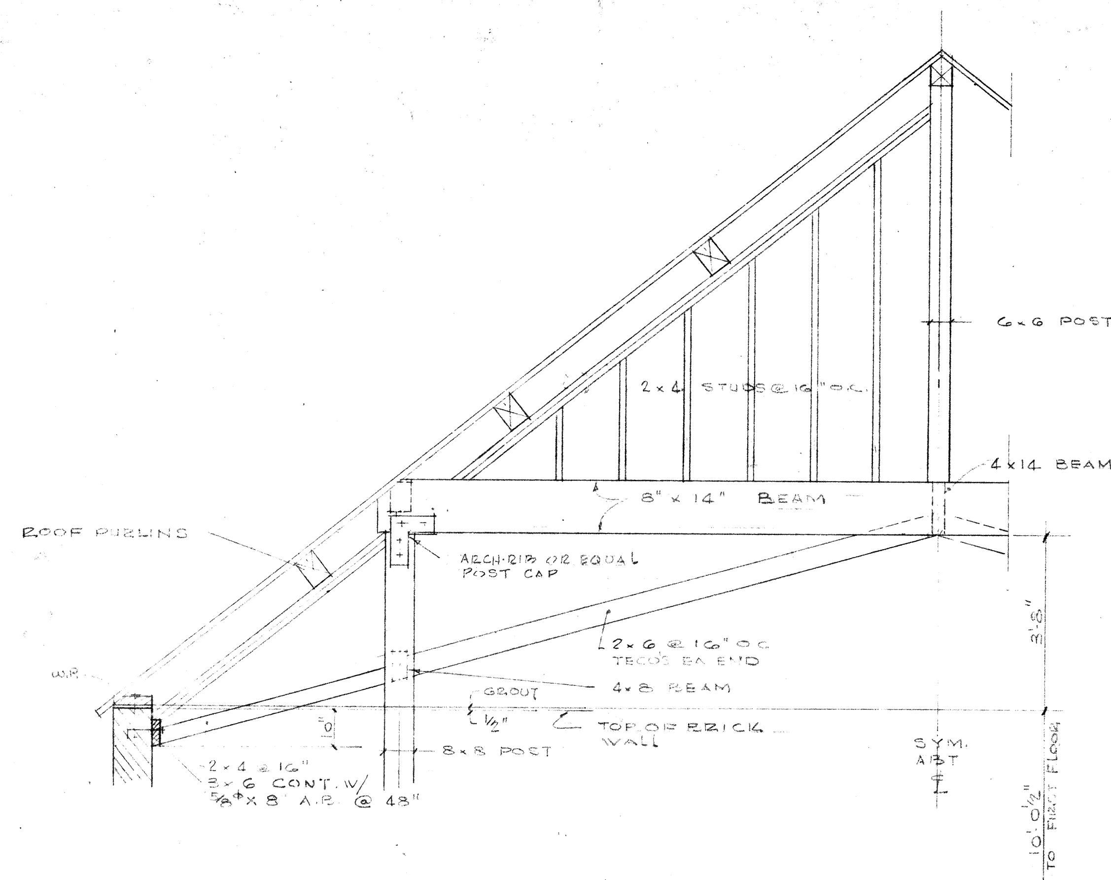
SECTION 1/2" = 1'-0"
