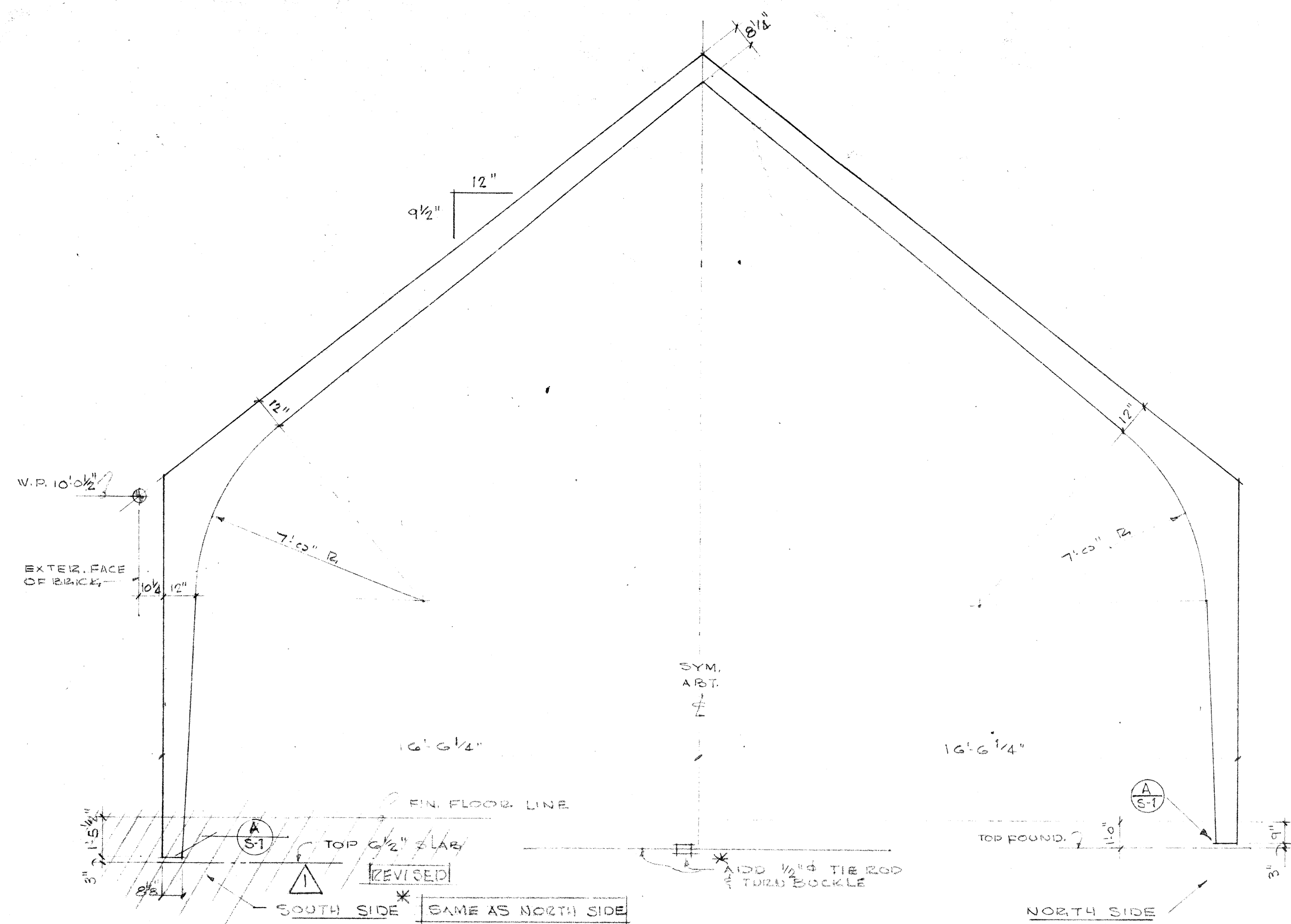
LAMINATED ARCH DETAIL
